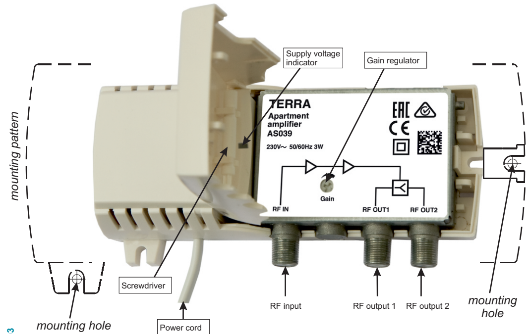
Figure 1. External view of the amplifier
